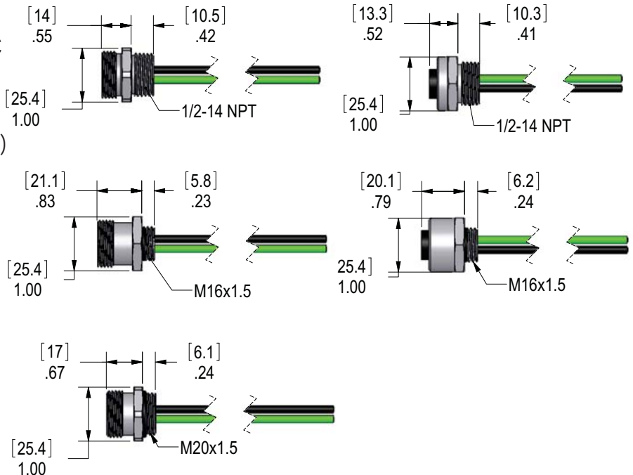
Male Receptacles
